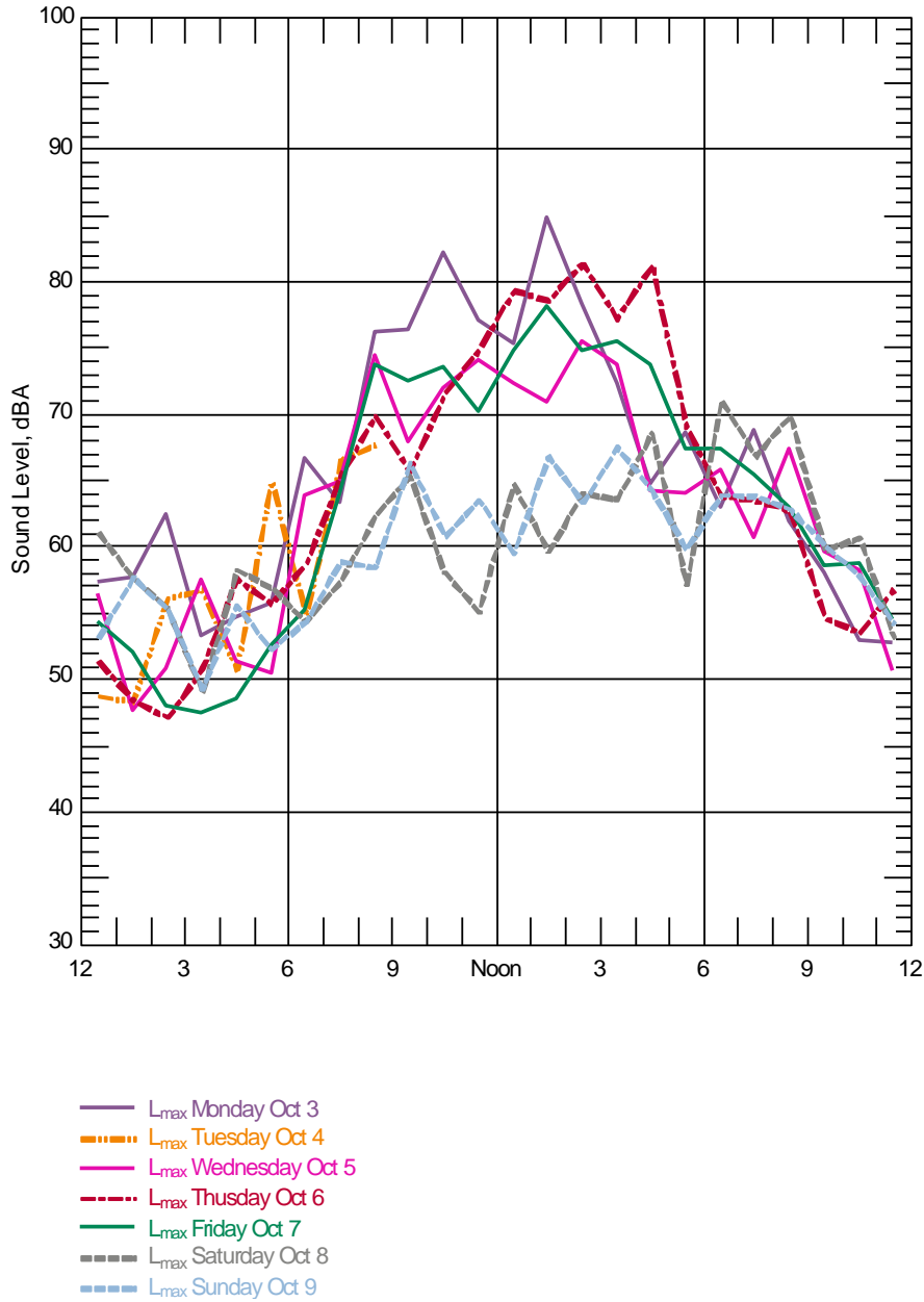
Figure 3: Hourly L max Noise Levels - NM1 (Hampel)
