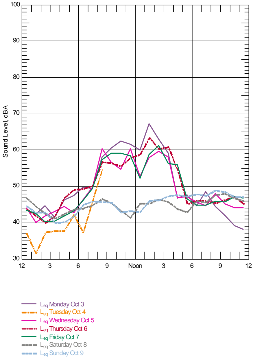
Figure 2: Hourly Energy Equivalent Noise Levels - NM1 (Hampel)
